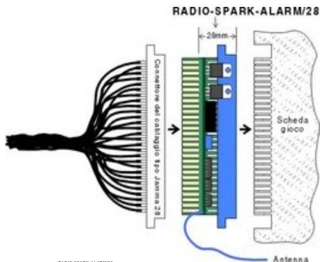
Art.A002 ...RADIO-SPARK-ALARM/28
