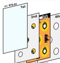
Composition of the EFT-1 front panel
