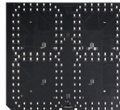
Art.0430-2522 F1502 LED board for INOUT-1s with 2 red digits Weight: 0,166kg.
